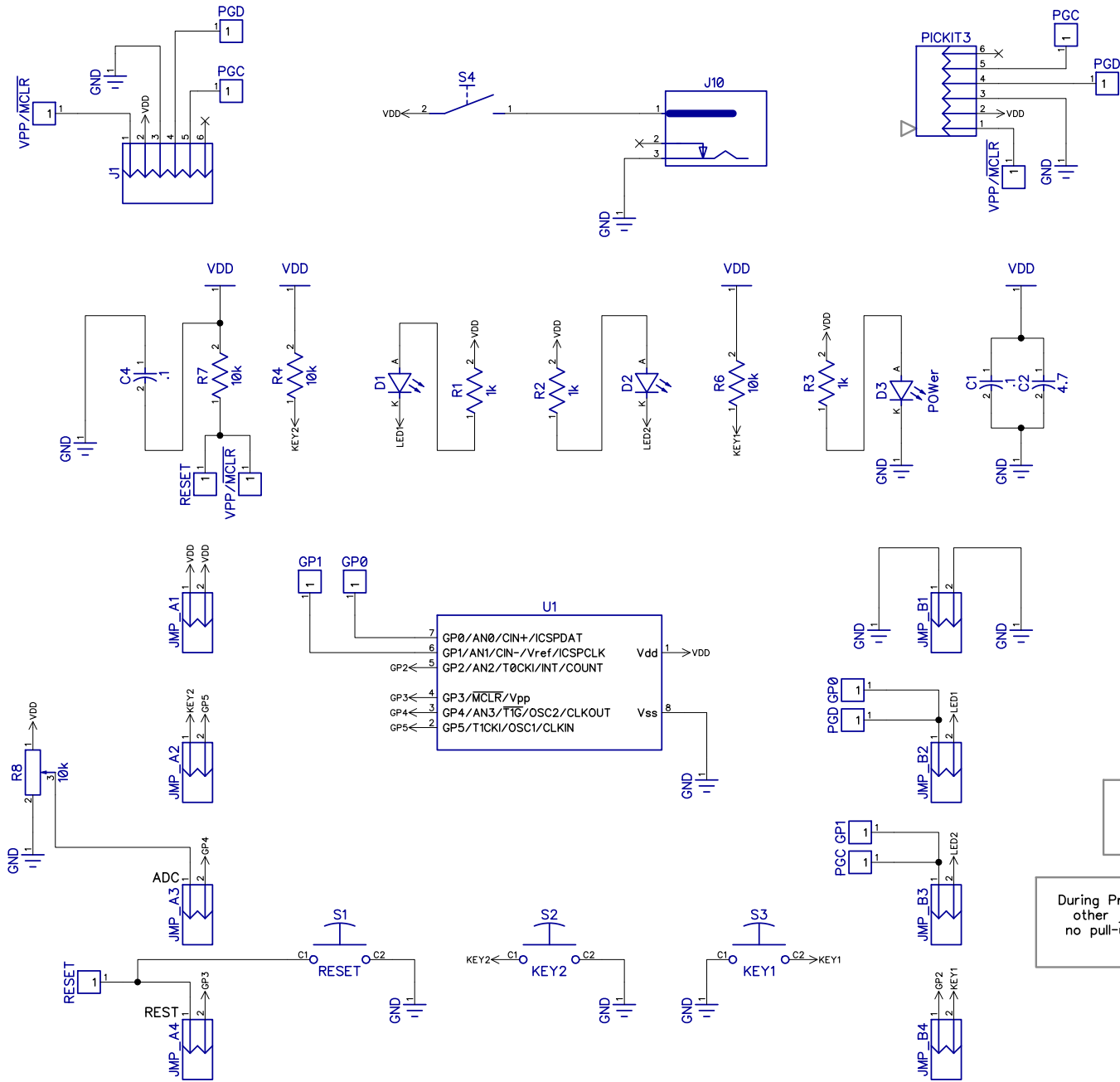
PIC12F675 Learning Board from EBAY Schematic drawn by Aardvark Labs
